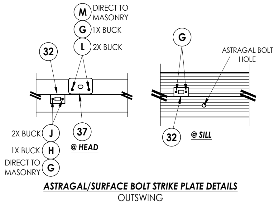
HARDWARE DETAILS
